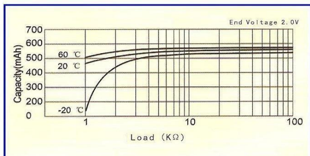
Load-capacity
