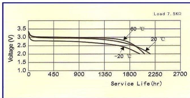
Temperature Characteristics
