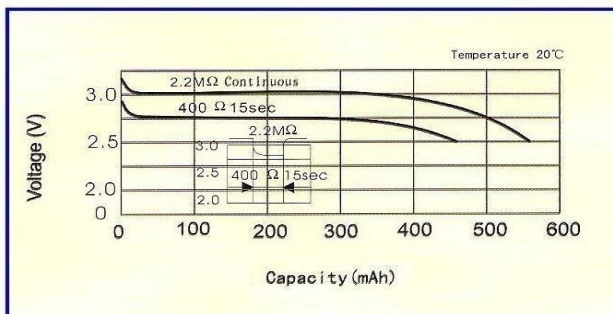
Pulse Discharge Characteristics
