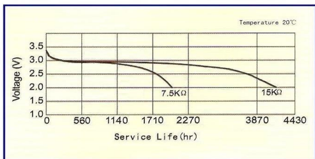
Discharge Characteristics
