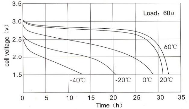
温度特性 Temperature Characteristics
